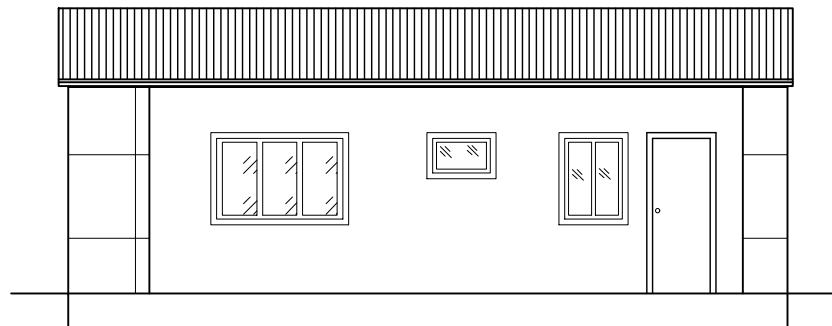
SOUTH ELEVATION
