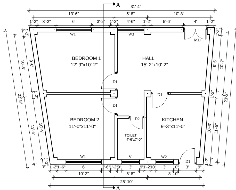
GROUND FLOOR PLAN AREA = 660.70 SQ.FT
